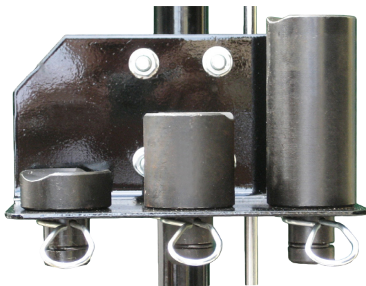
Saddle Kit
