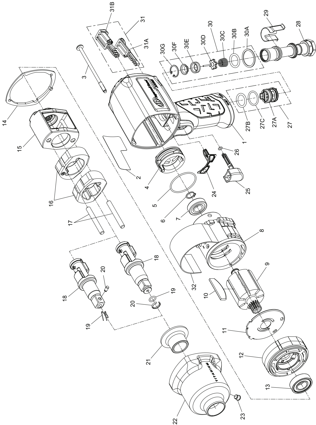
Figure 1. Exploded View - 47517574
