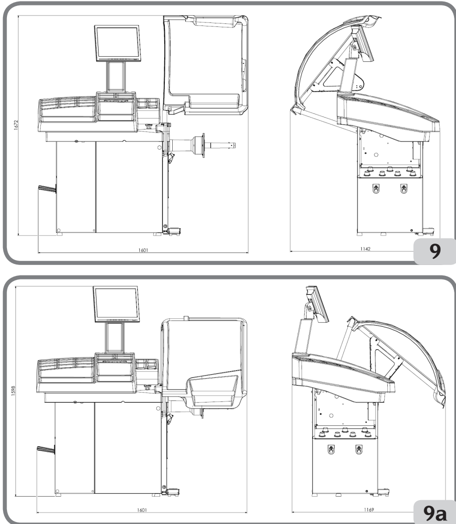
Machine dimensions (Fig. 9/9a)
