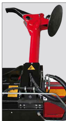
Automatic lift and rotate action for tool holder arm and bead breaker disc.
