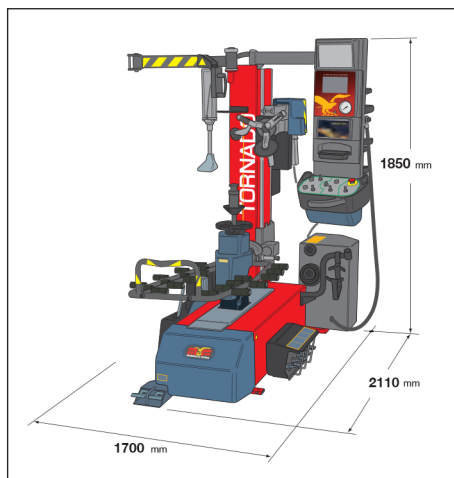
Dimension of Tornado Tire Changer With Premium Lift
